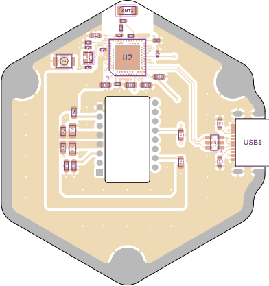
Top Assembly (Scale 1:1)
